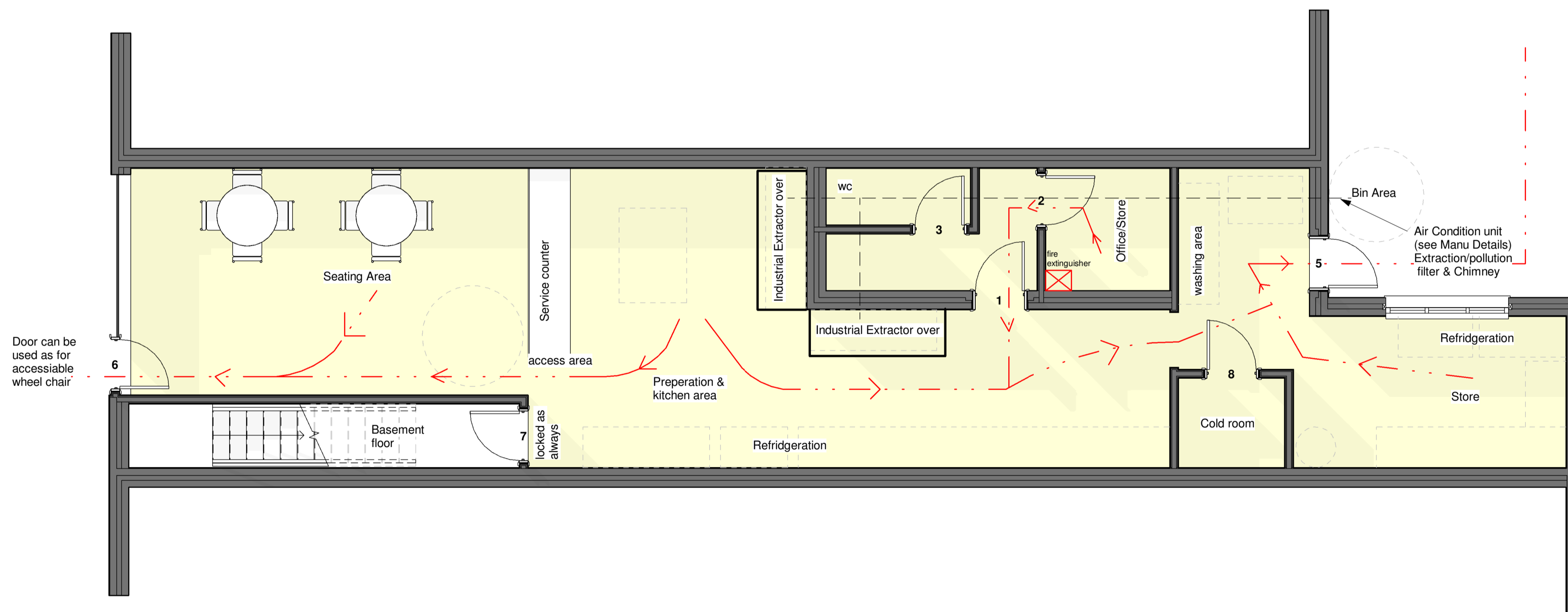
2 00 - GROUND FLOOR PLAN - Fire Plan 1 : 50
