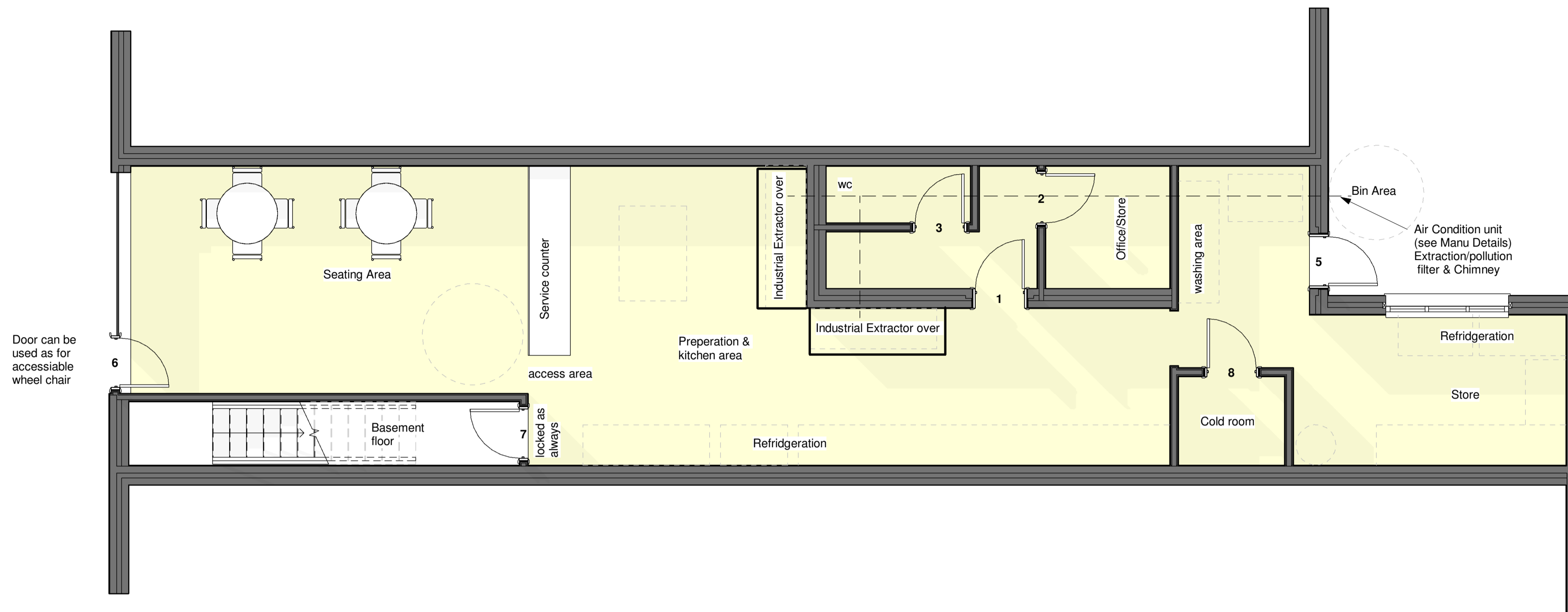
1 00 - GROUND FLOOR PLAN 1 : 50
